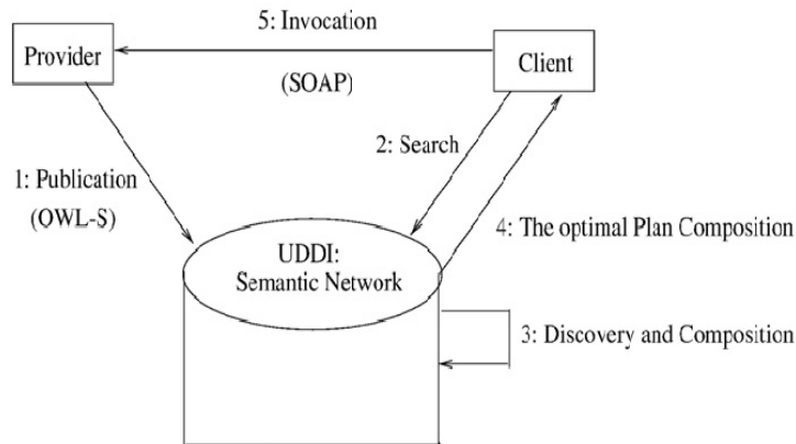
Figure 28.1. Architecture des Web services.
