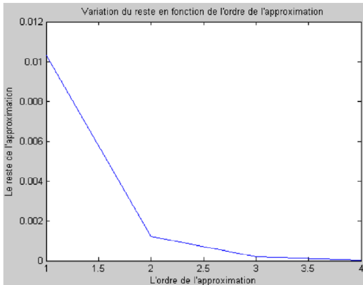
Figure 12.5. Variation of the Reminder Term
