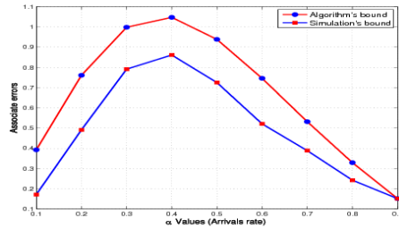
Figure 2.1. Comparative curves of the approximation errors : case Cox_2 law.
