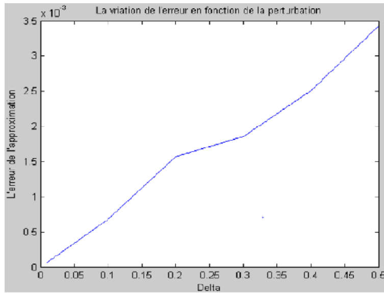
Figure 12.6. Variation of the approximation error
