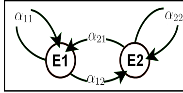
Figure 5.1. Transition's graph of the \{\tilde{X}(t), t \geq 0\} process.
