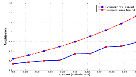
Figure 2.2. Comparative curves of the approximation errors : case E_2 law.
