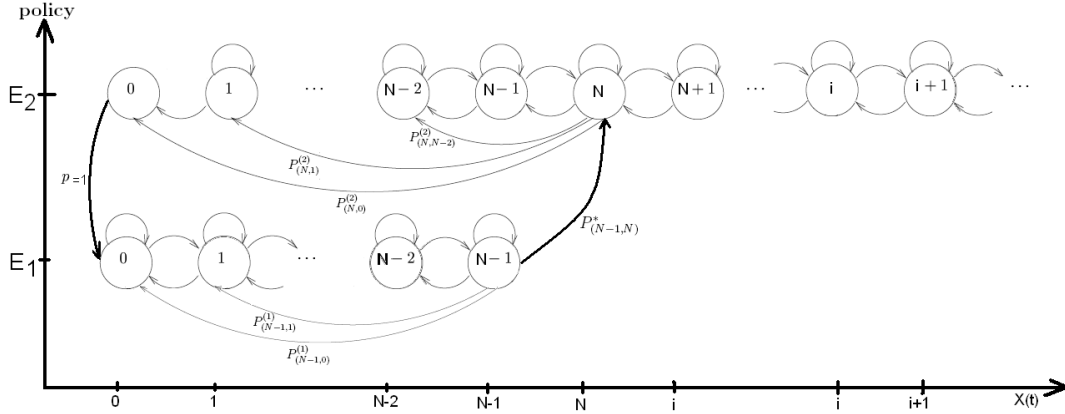
Figure 5.2. Transition's graph of the \{\tilde{X}_n, n \geq 1\} process.
