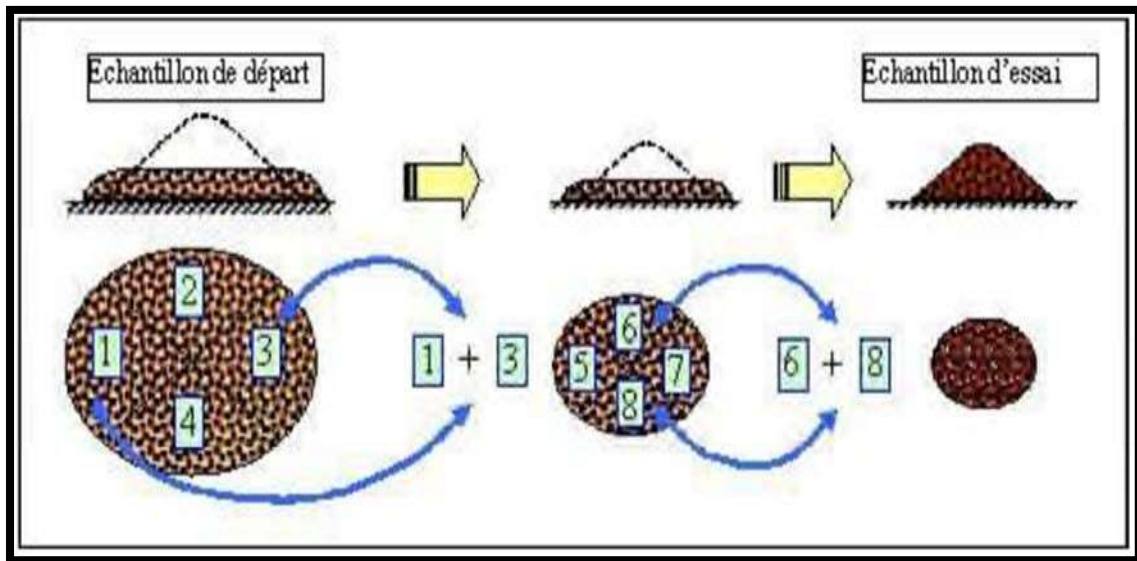
Figure II.6. Principe de quartage.
