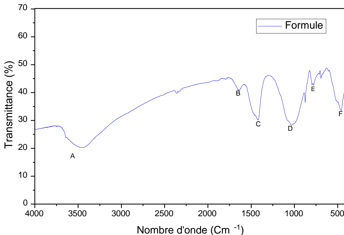
Figure III.4. Spectre infrarouge de la formulation.
