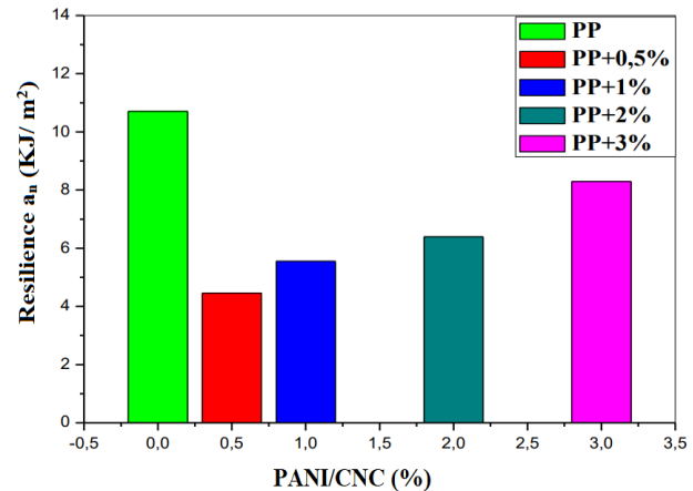
Figure 5. Variations of impact strength for PP/PANI-CNC nanocomposites versus PANI-CNC content
