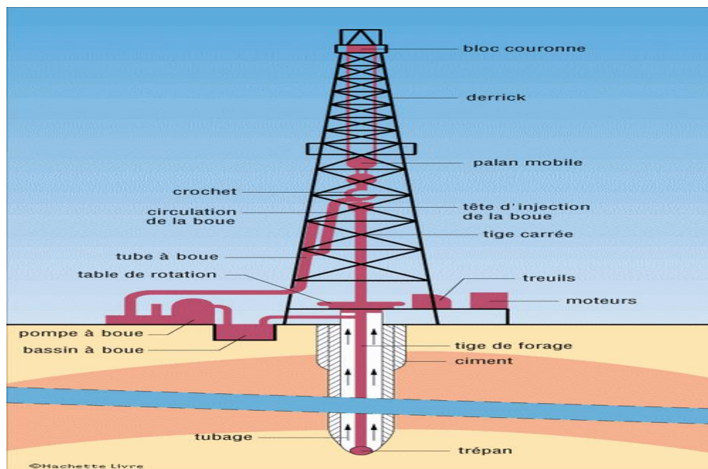
Figure 1: Forage verticale [2]
